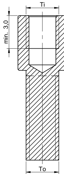
sectional drawing A-A
